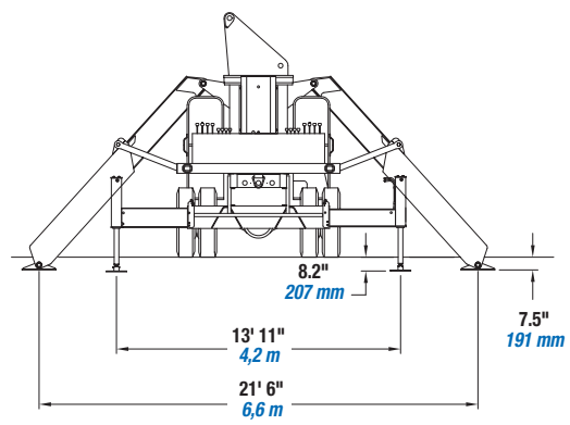
Out-Down Rear Stabilizers (option)
